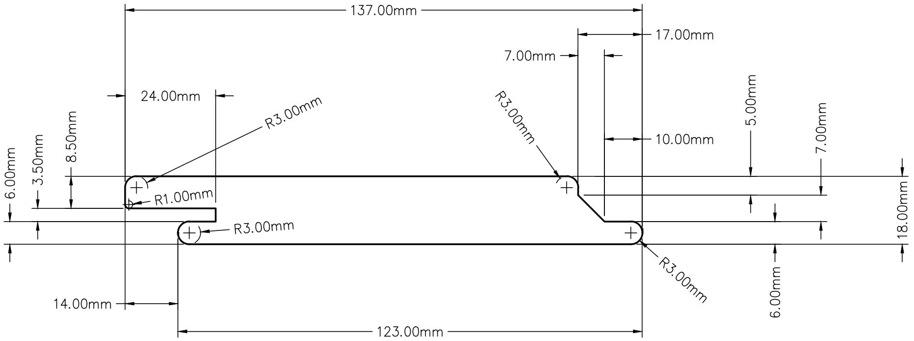
1 SIDE PROFILE 18MMx137MM 2A SCALE 1:1
